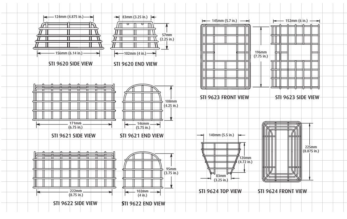
▼ Motion Detector Cages dimensions and technical information (STI 9620, STI 9621, STI 9622, STI 9623 & STI 9624)
